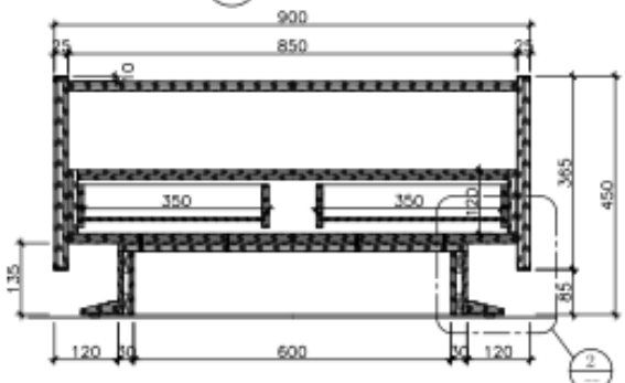
(F) Side View 1:10
