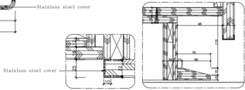
(1) Detailed structure 1:3
