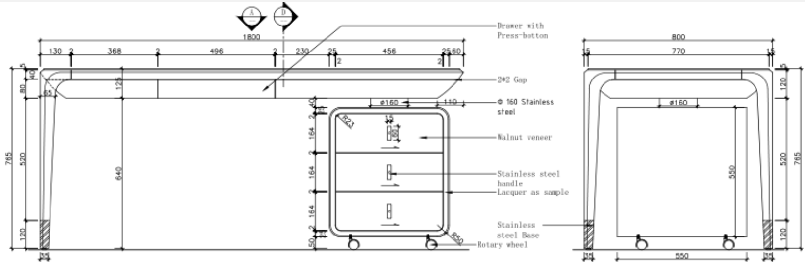
(B) Front View 1:10
